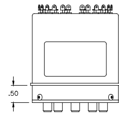
HS SWITCH
