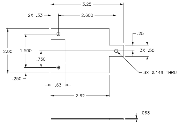
“G” BRACKET
