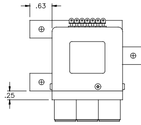
TN/TNH SWITCH
