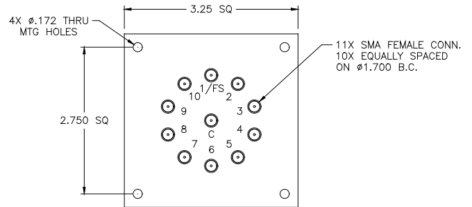
HS SWITCH
