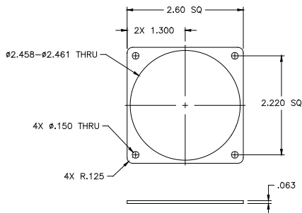
“H” BRACKET
