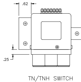
TN/TNH SWITCH
