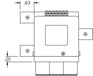
TT SWITCH
